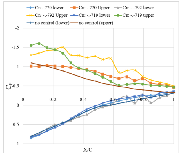
Fig.10: Pressure coefficient distribution for controlled case. Angle of attack 10°. Leading edge excitation
