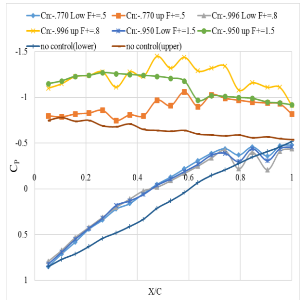
Fig.9: Pressure coefficient distribution for controlled case. Angle of attack 15°. Leading edge excitation.
