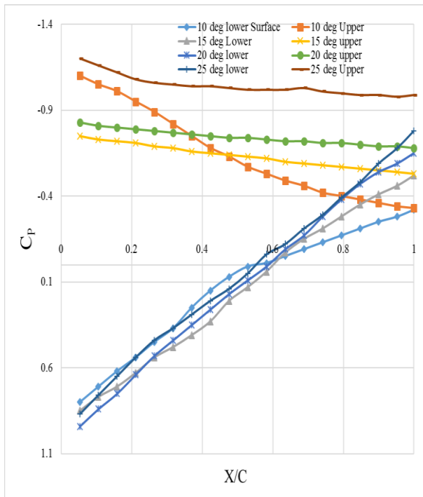
Fig.6: Airfoil pressure coefficient distribution at different angles of attack. Suction and pressure sides. No actuation.
