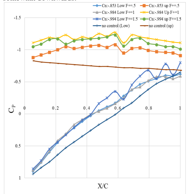
Fig 7: Pressure coefficient distribution for controlled case. Angle of attack at 20°, Leading edge excitation.
