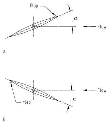
Figure 5. Schematic of flap positions tested. a) Leading edge flap; b) trailing edge flap.
