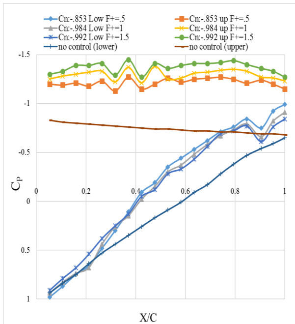
Fig.8: Pressure coefficient distribution for controlled case. Angle of attack 20°. Trailing edge excitation.
